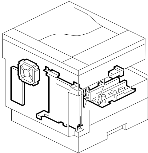
17. ELECTRICAL SECTION
